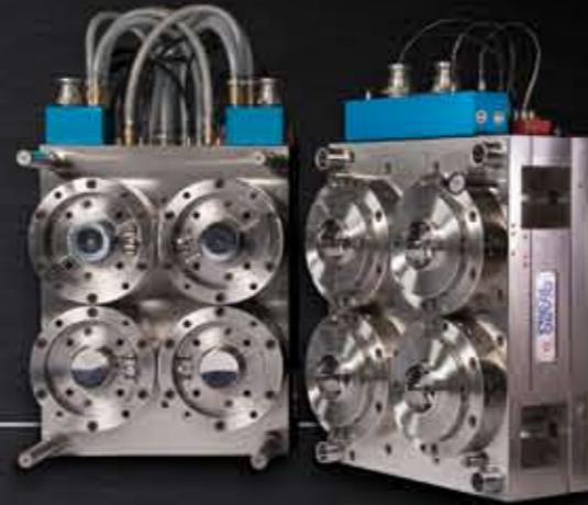
4 fach Dose 280 ml 4 cavity tub 280 ml
