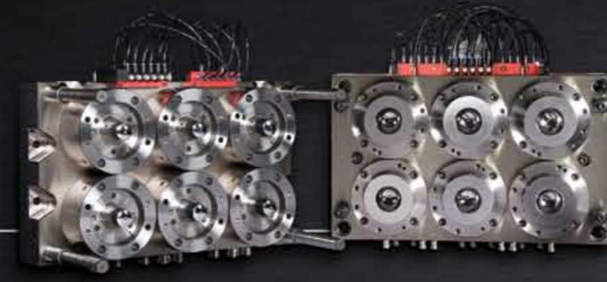
6 fach Fussbecher 150 ml 6 cavity cup with foot 150 ml
